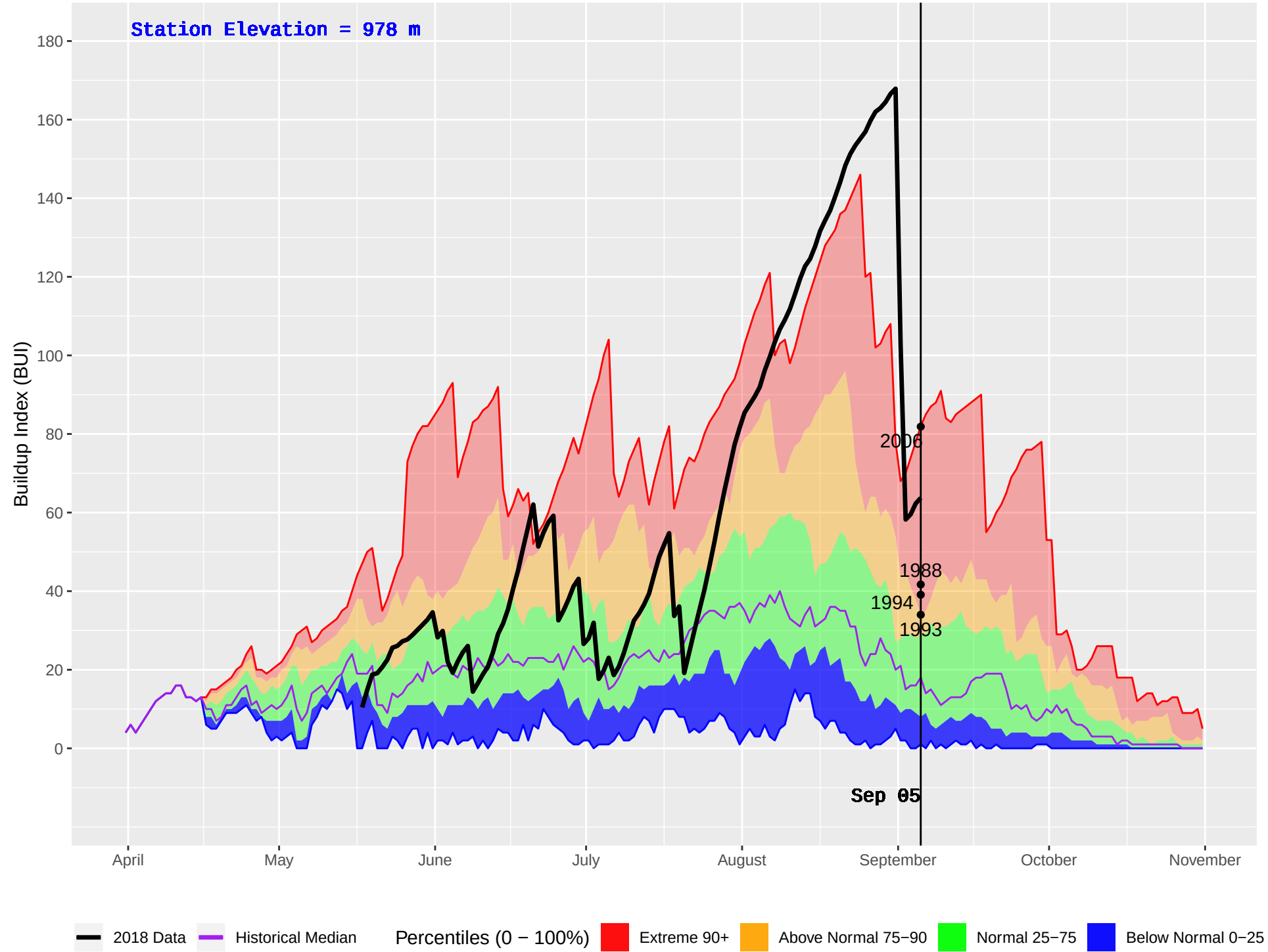
NILKITKWA (172) : Historical (1986–2016) and Current (2018) Daily Buildup Index (BUI)
